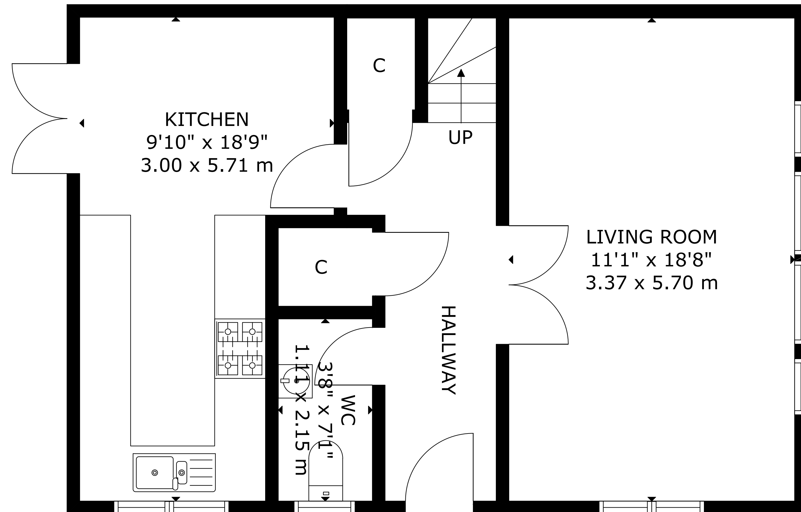
GROUND FLOOR
