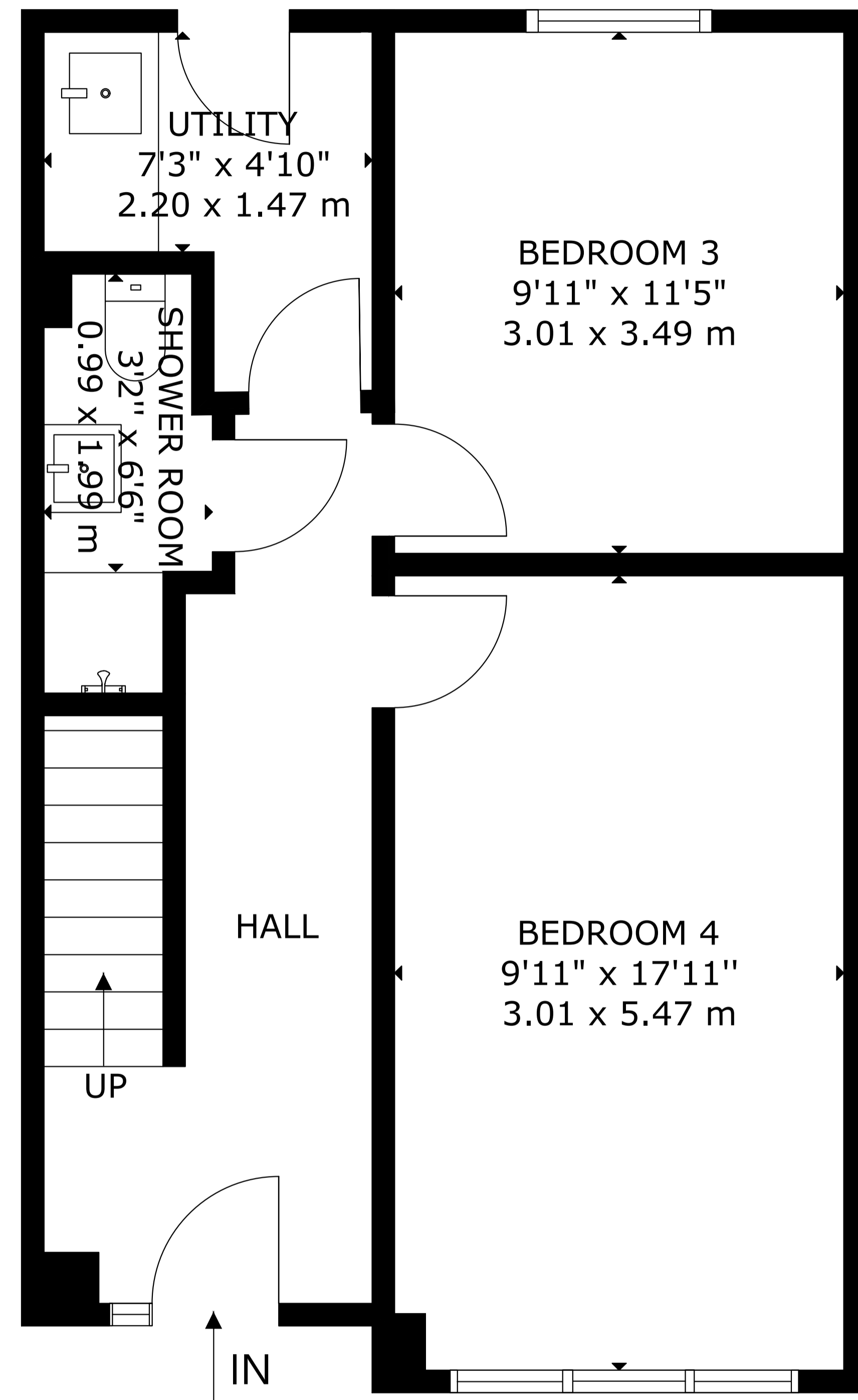
GROUND FLOOR
