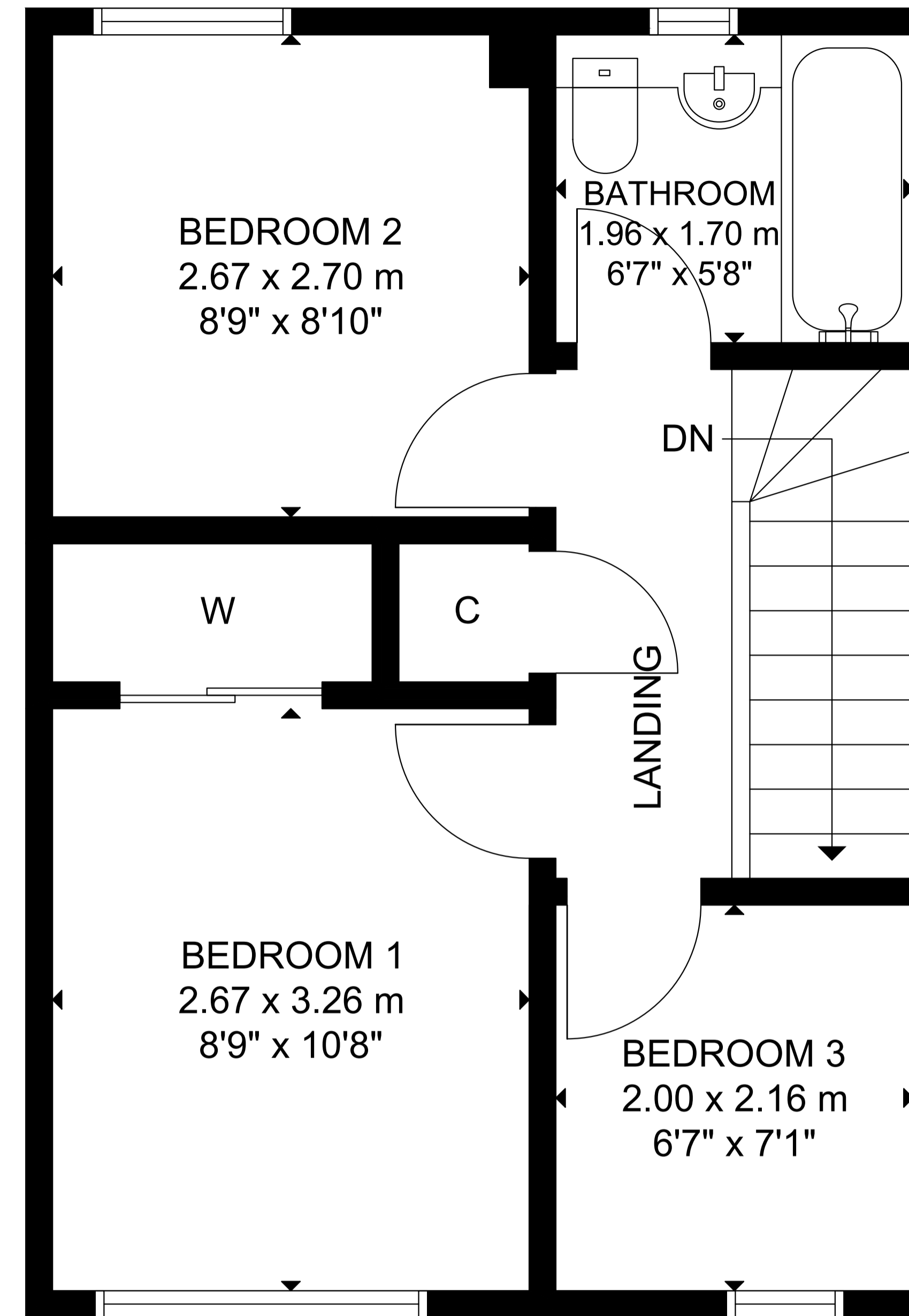
FIRST FLOOR
